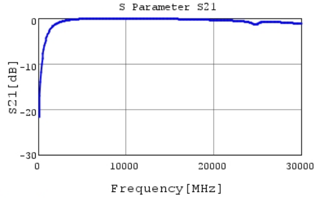
GJM0335C1E1R3WB01 S21 DCOV, 25degC
