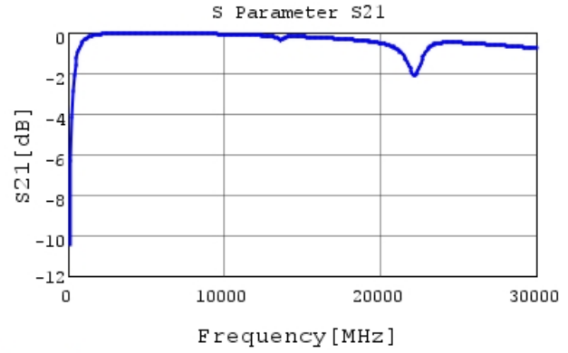
GJM0335C1E5R0WB01 S21 DCOV, 25degC
