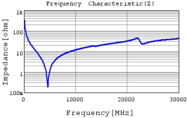
GJM0335C1E5R0WB01 |Z| DCOV, 25degC
