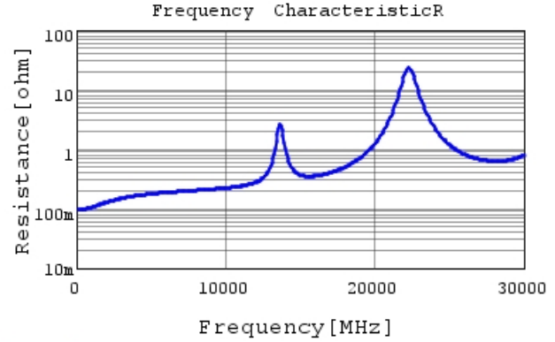
GJM0335C1E5R0WB01 R DCOV, 25degC
