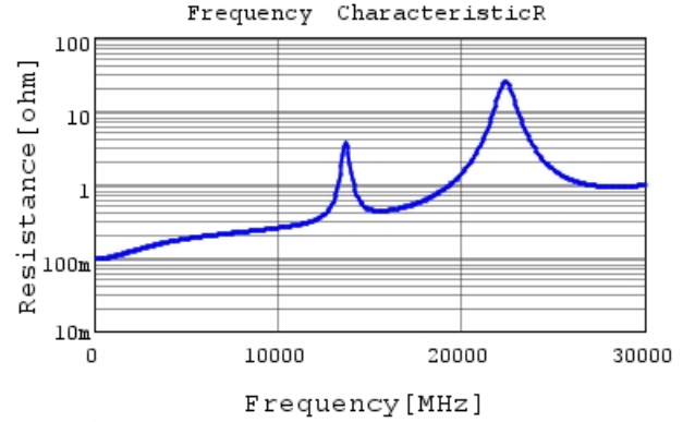
GJM0335C1E4R7WB01 R DCOV, 25degC
