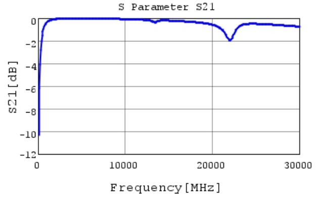
GJM0335C1E5R1WB01 S21 DCOV, 25degC
