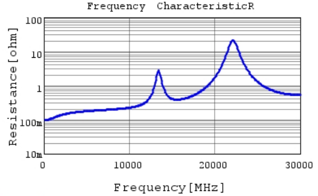
GJM0335C1E5R1WB01 R DCOV, 25degC
