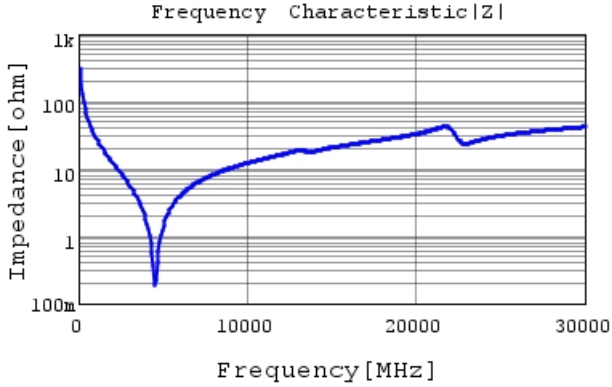
GJM0335C1E5R1WB01 |Z| DCOV, 25degC
