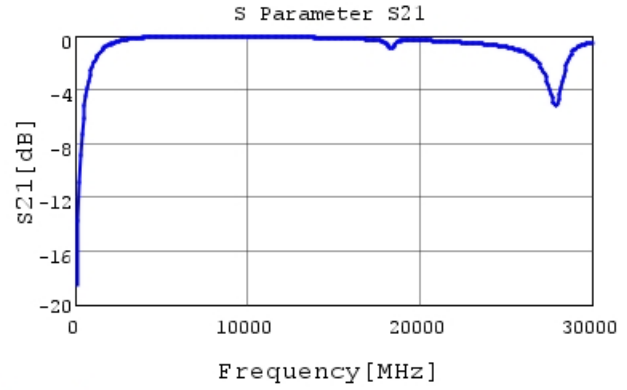
GJM0335C1E1R9WB01 S21 DCOV, 25degC
