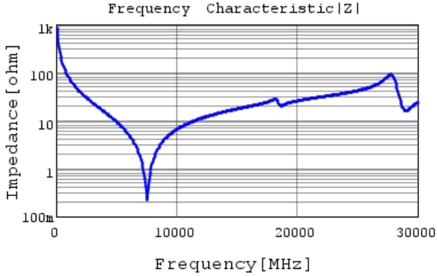
GJM0335C1E1R9WB01 |Z| DCOV, 25degC
