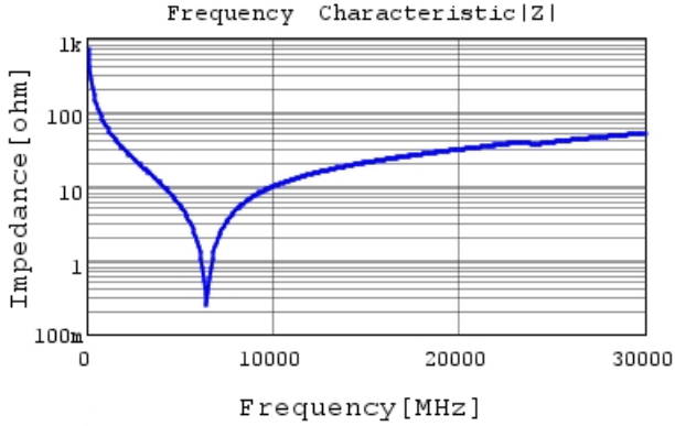
GJM0335C1E2R3WB01 |Z| DCOV, 25degC
