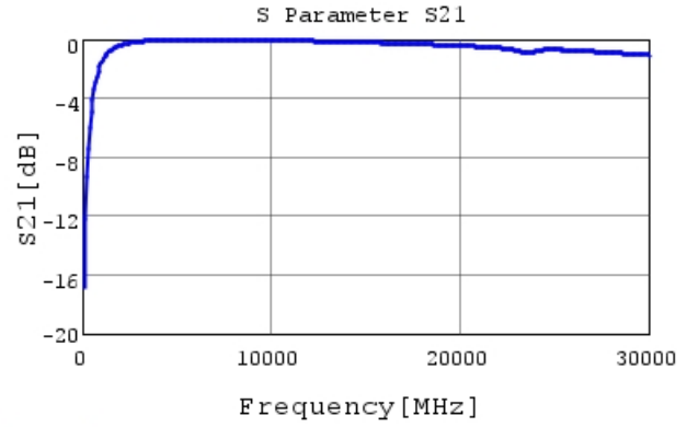
GJM0335C1E2R3WB01 S21 DCOV, 25degC
