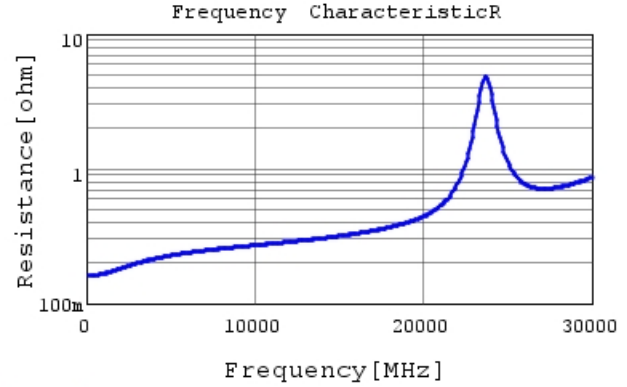
GJM0335C1E2R3WB01 R DCOV, 25degC
