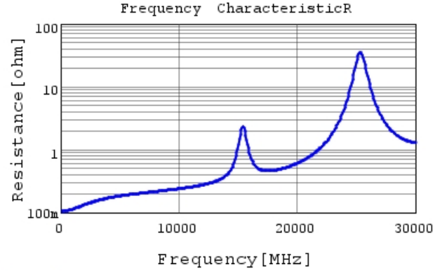
GJM0335C1E3R9WB01 R DCOV, 25degC
