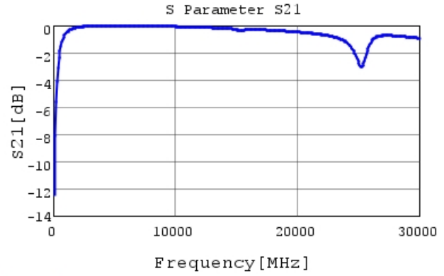
GJM0335C1E3R9WB01 S21 DCOV, 25degC
