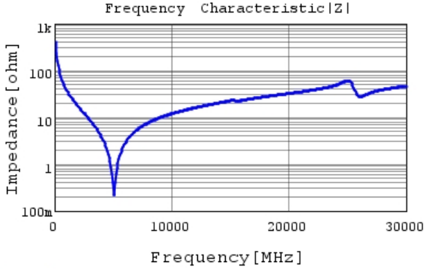
GJM0335C1E3R9WB01 |Z| DCOV, 25degC
