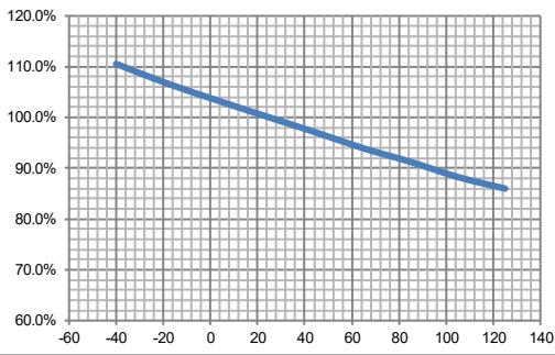
Derating Curve
