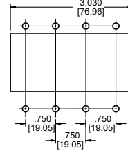
MountingDetail*
