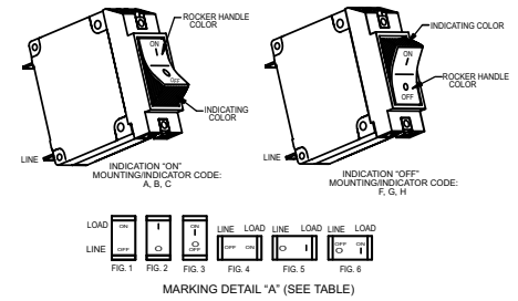
MARKING DETAIL "A" (SEE TABLE)
