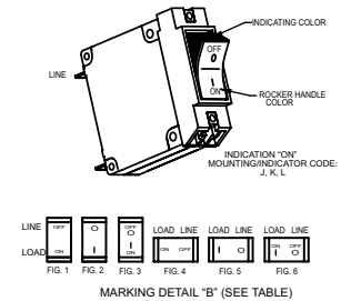
MARKING DETAIL "B" (SEE TABLE)
