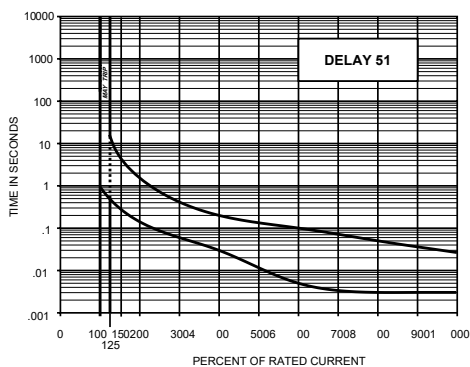
DC Delay Curves (typ)
