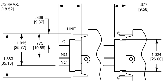
Series with Auxiliary Switch
