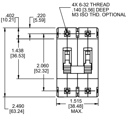
Two Pole*
