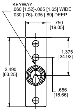
Single Pole
