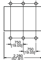
Mounting Detail*
