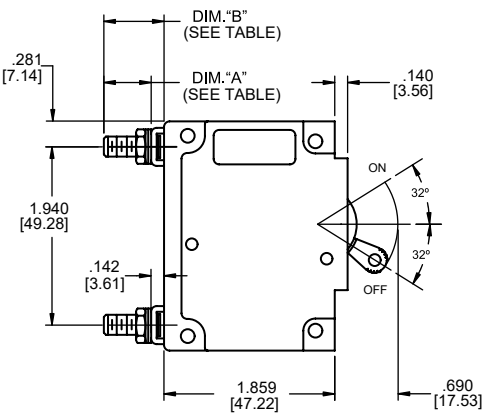
Two Pole
