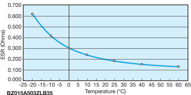
ESR vs. Temperature
