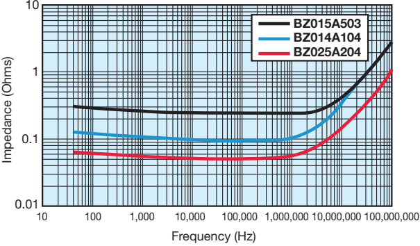
Impedance Comparison
