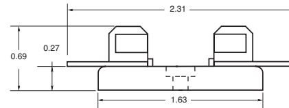
4405 0° integral solder terminals clips
