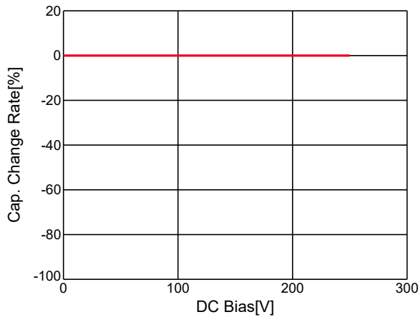
GQM2195G2E151GB12#,C-DC bias,capchange, 25.0degC, AC1Vrms
