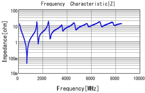
GQM2195G2E121JB12 |Z| DCOV, 25degC
