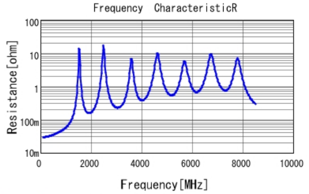
GQM2195G2E121JB12 R DCOV, 25degC
