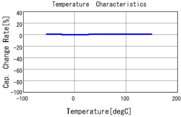
GQM2195G2E121JB12 C-Temp. capchange, DCOV, AC1Vrms
