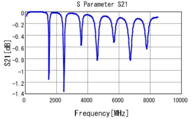
GQM2195G2E121JB12 S21 DCOV, 25degC
