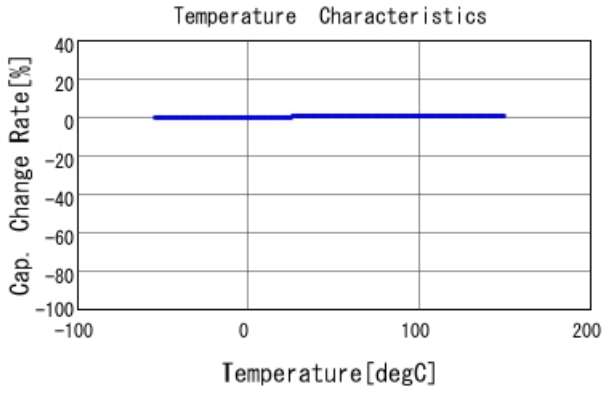
■ GQM1875G2E9R1BB12 C-Temp. capchange, DCOV, AC1Vrms
