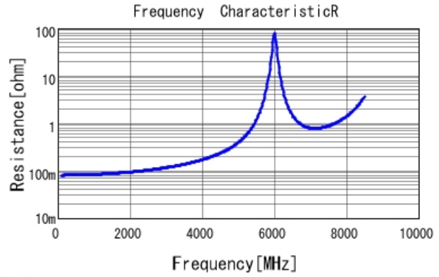
■ GQM1875G2E9R1BB12 R DCOV, 25degC
