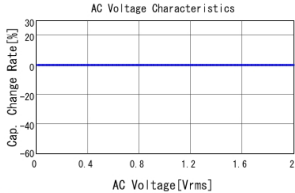
■ GQM1875G2E9R1BB12 C-AC Voltage capchange, DCOV, 25.0d
