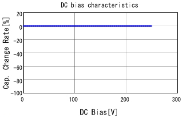
■ GQM1875G2E9R1BB12 C-DC bias capchange, 25.0degC, AC1V
