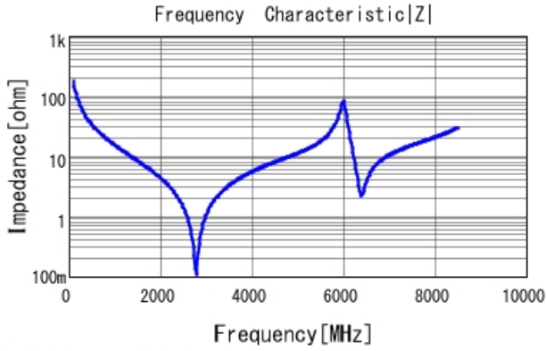
■ GQM1875G2E9R1BB12 |Z| DCOV, 25degC
