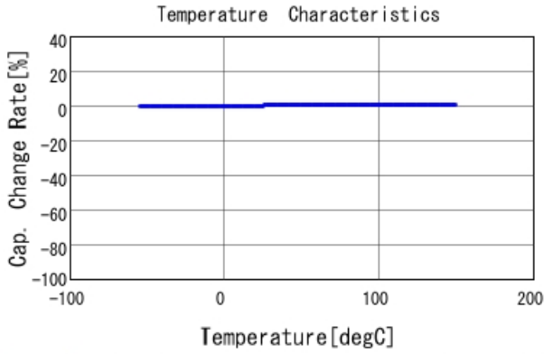
GQM1875G2E3R6BB12 C-Temp. capchange, DCOV, AC1Vrms
