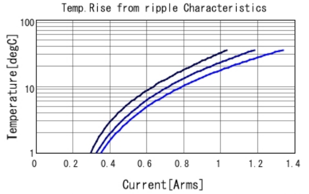
GQM1875G2E3R6BB12 Temp. rise — 1GHz — 2GHz
