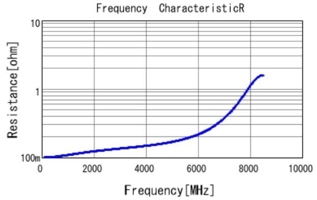
GQM1875G2E3R6BB12 R DCOV, 25degC
