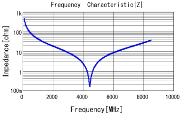
GQM1875G2E3R6BB12 |Z| DCOV, 25degC
