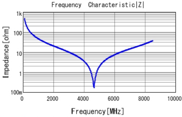
GQM1875G2E3R3WB12 |Z| DCOV, 25degC
