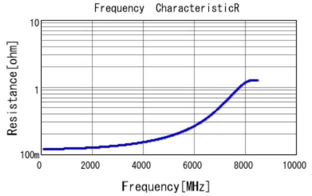
GQM1875G2E3R3WB12 R DCOV, 25degC
