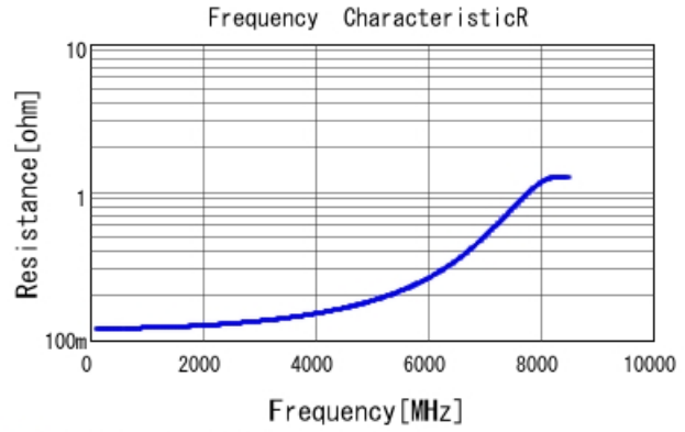
■ GQM1875G2E3R3BB12 R DCOV, 25degC
