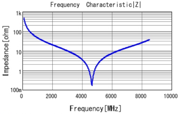
■ GQM1875G2E3R3BB12 |Z| DCOV, 25degC
