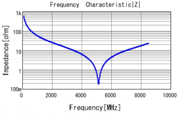
GQM1875G2E2R7WB12 |Z| DCOV, 25degC
