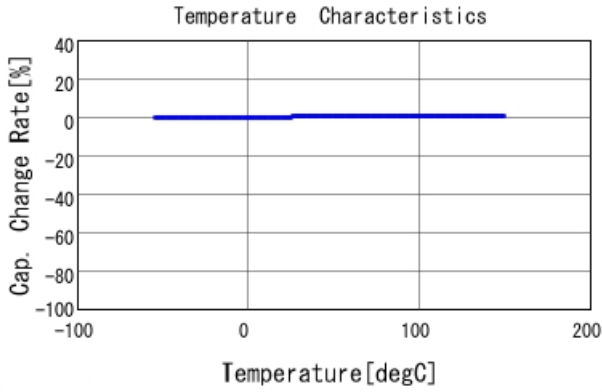
GQM1875G2E2R7WB12 C-Temp. capchange, DCOV, AC1Vrms
