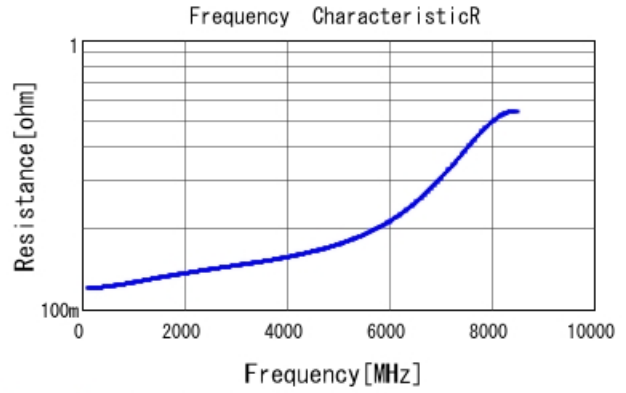
GQM1875G2E2R7WB12 R DCOV, 25degC
