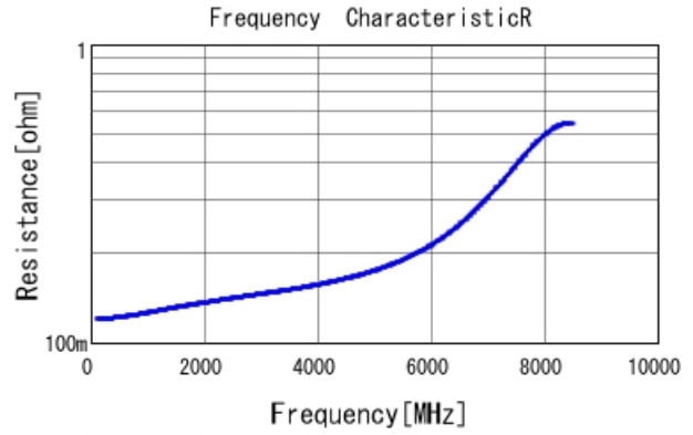
GQM1875G2E2R7BB12 R DCOV, 25degC
