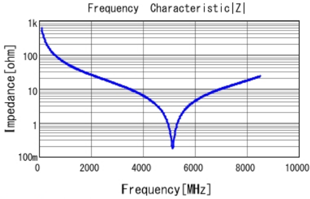
GQM1875G2E2R7BB12 |Z| DCOV, 25degC
