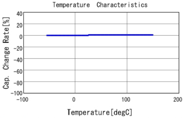
GQM1875G2E2R7BB12 C-Temp. capchange, DCOV, AC1Vrms
