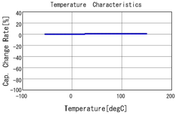
■ GQM1875G2E1R8BB12 C-Temp. capchange, DCOV, AC1Vrms
