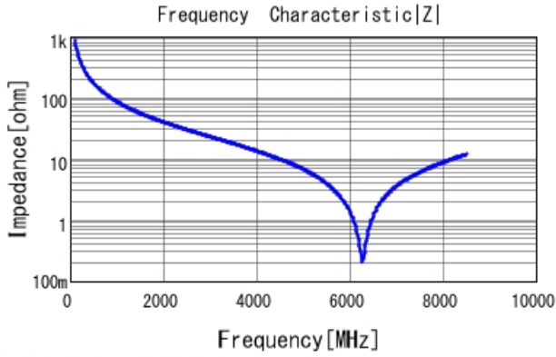
■ GQM1875G2E1R8BB12 |Z| DCOV, 25degC
