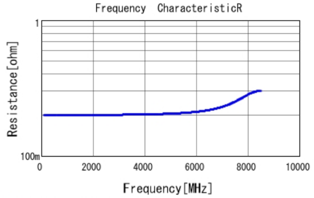
■ GQM1875G2E1R8BB12 R DCOV, 25degC
