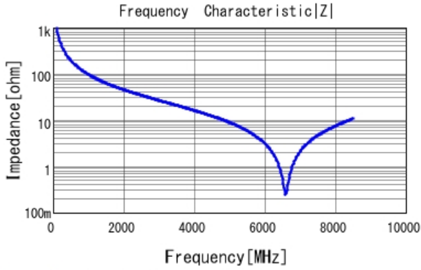
GQM1875G2E1R6WB12 |Z| DCOV, 25degC
