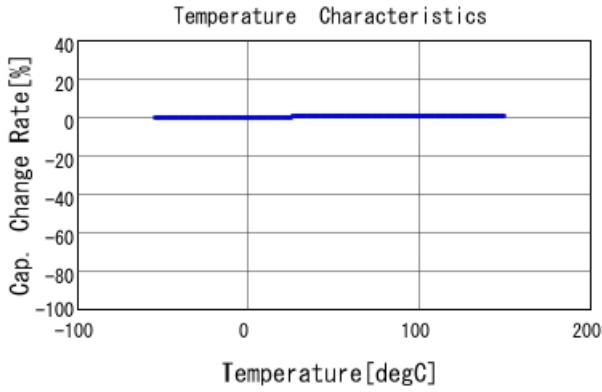
GQM1875G2E1R6WB12 C-Temp. capchange, DCOV, AC1Vrms
