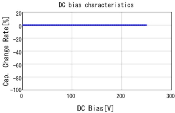
GQM1875G2E1R6WB12 C-DC bias capchange, 25.0degC, A
