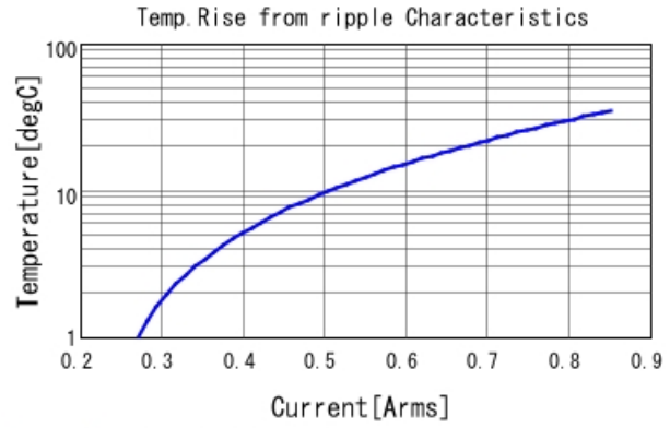
GQM1875G2E1R0WB12 Temp. rise 3GHz
