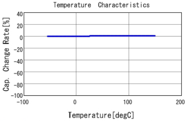
GQM1875G2E1R0WB12 C-Temp. capchange, DCOV, AC1Vrms
