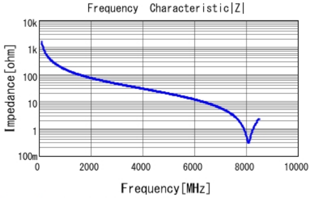
GQM1875G2E1R0WB12 |Z| DCOV, 25degC
