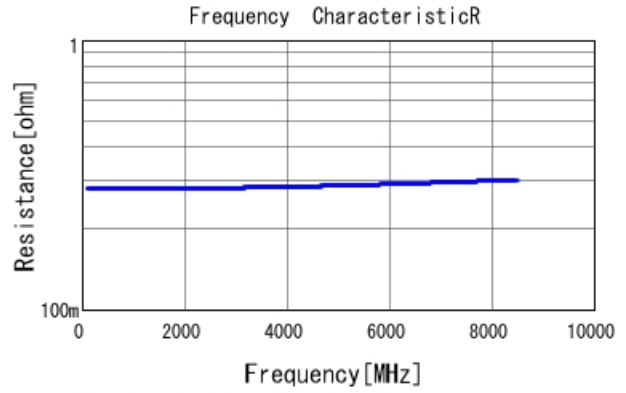
GQM1875G2E1R0WB12 R DCOV, 25degC
