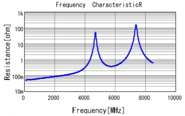
■ GQM1875G2E150JB12 R DC0V, 25degC
