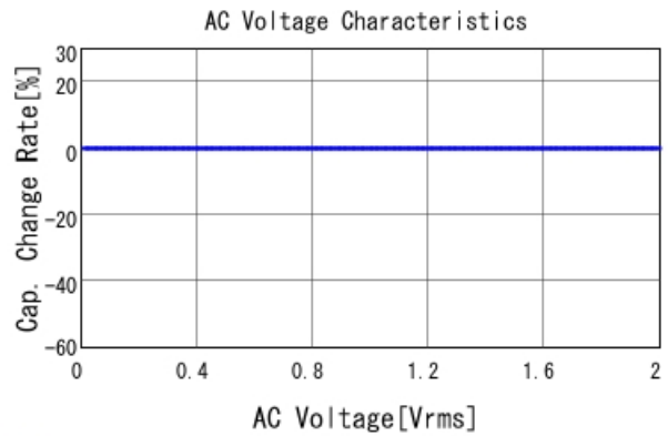
■ GQM1875G2E150JB12 C-AC Voltage capchange, DC0V, 25.0d
