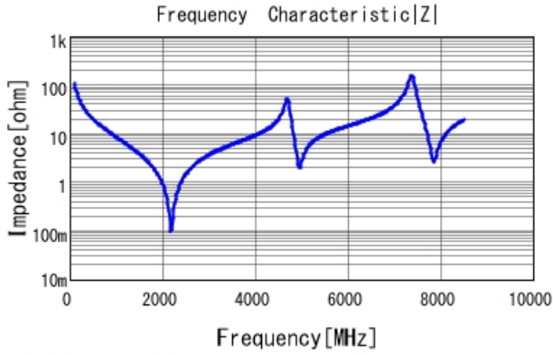
■ GQM1875G2E150JB12 |Z| DC0V, 25degC
