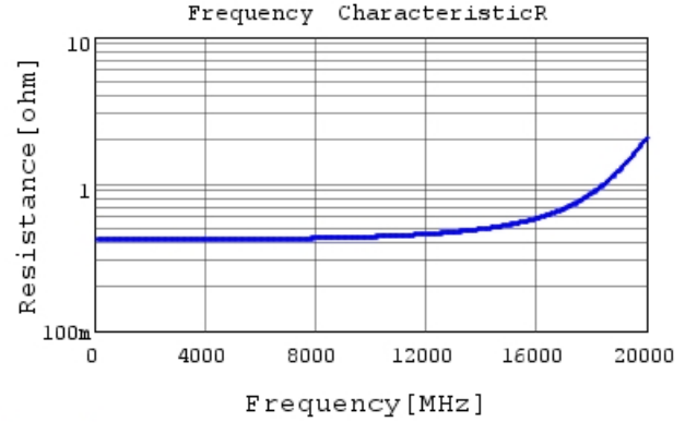
GJM1555C1HR30BB01 R DCOV, 25degC
