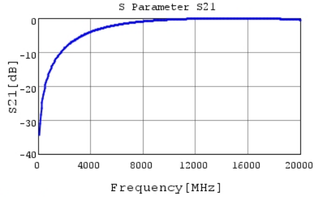
GJM1555C1HR30BB01 S21 DCOV, 25degC
