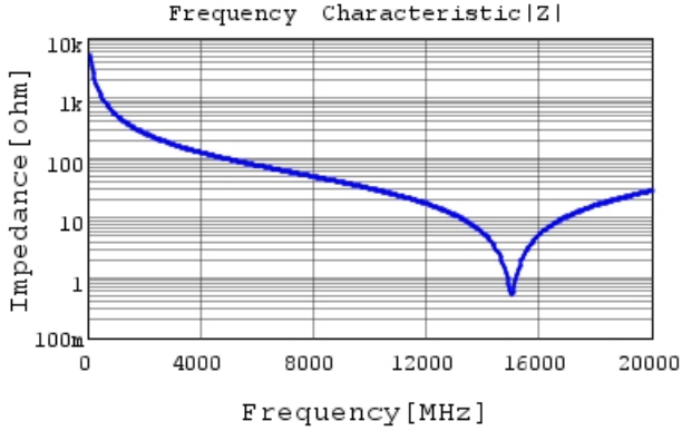
GJM1555C1HR30BB01 |Z| DCOV, 25degC
