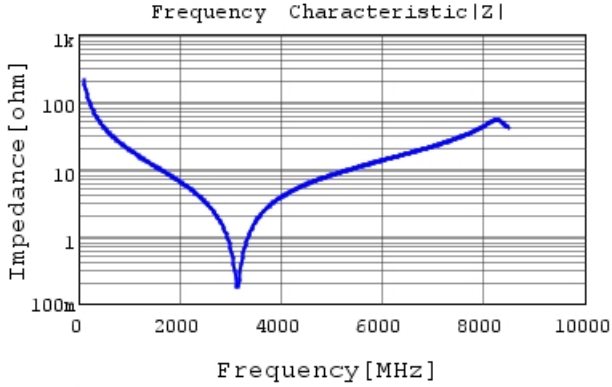
GJM1555C1H7R5CB01 |Z| DC0V, 25degC
