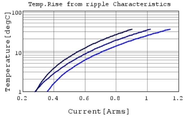
GJM1555C1H7R5CB01 Temp.rise 1GHz 2
