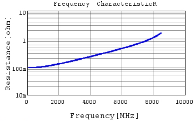
GJM1555C1H6R2DB01 R DC0V, 25degC
