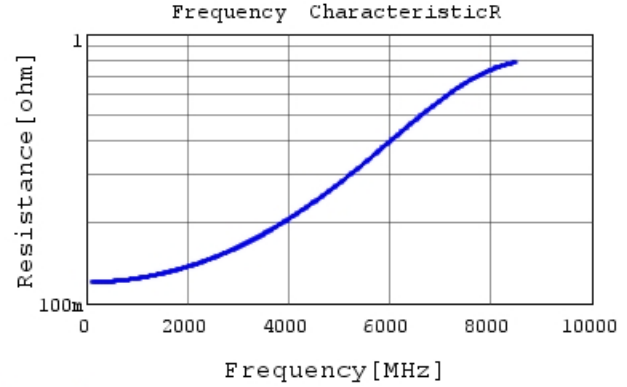
GJM1555C1H4R0BB01 R DCOV, 25degC
