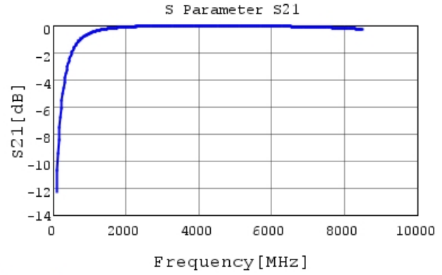
GJM1555C1H4R0BB01 S21 DCOV, 25degC
