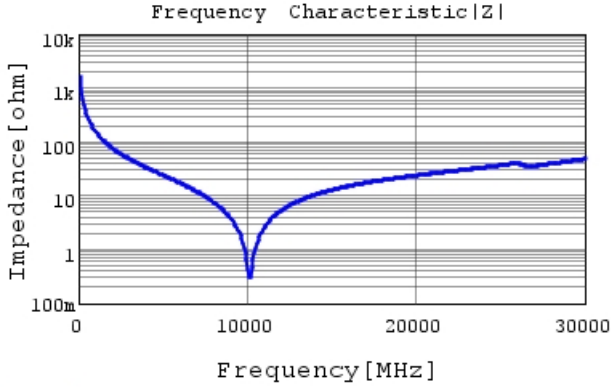
GJM0335C1H1R0BB01 |Z| DCOV, 25degC
