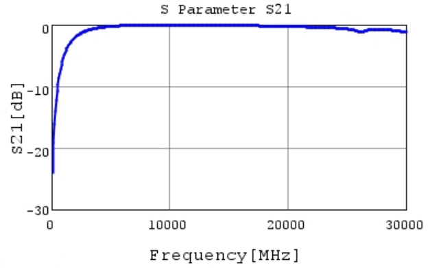
GJM0335C1H1R0BB01 S21 DCOV, 25degC
