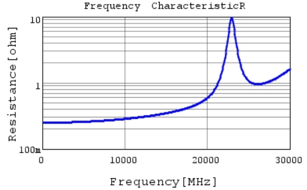
GJM0335C1E1R5WB01 R DCOV, 25degC
