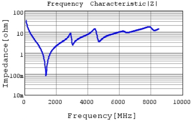
GCQ1555C1H470GB01 |Z| DC0V, 25degC
