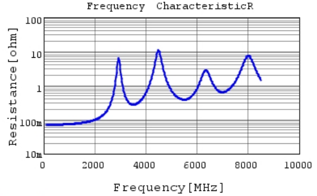
GCQ1555C1H470GB01 R DC0V, 25degC
