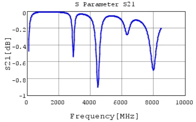
GCQ1555C1H470GB01 S21 DCOV, 25degC
