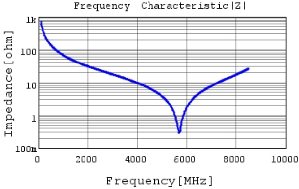
GCQ1555C1H2R3WB01 |Z| DC0V, 25degC
