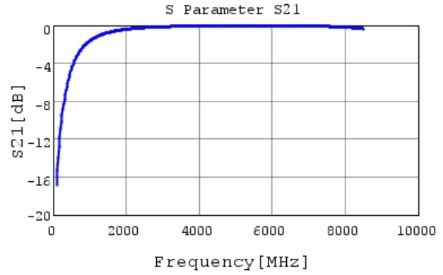
GCQ1555C1H2R3WB01 S21 DCOV, 25degC
