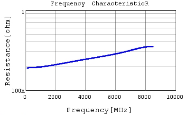
GCQ1555C1H2R1WB01 R DC0V, 25degC
