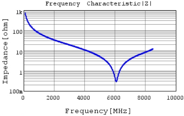
GCQ1555C1H2R1WB01 |Z| DC0V, 25degC
