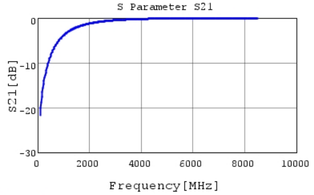
GCQ1555C1H1R3WB01 S21 DCOV, 25degC
