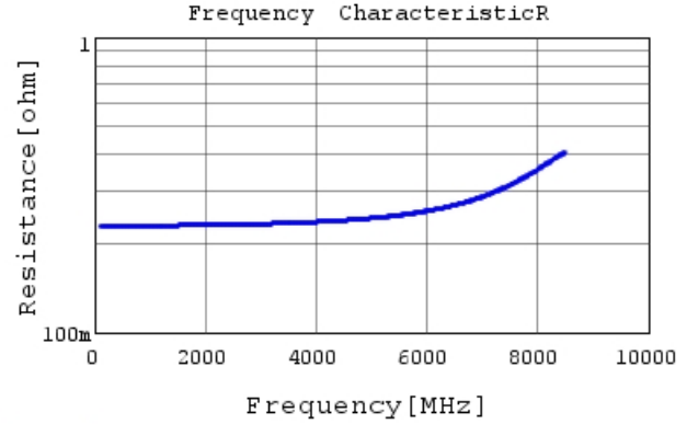
GCQ1555C1H1R3WB01 R DC0V, 25degC
