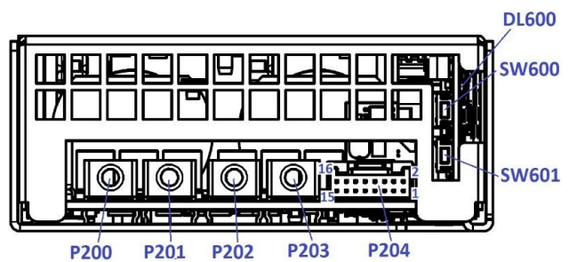
Figure 7. Rear View - ACC750-1T24-PC / ACC750-1T48-PC Models
