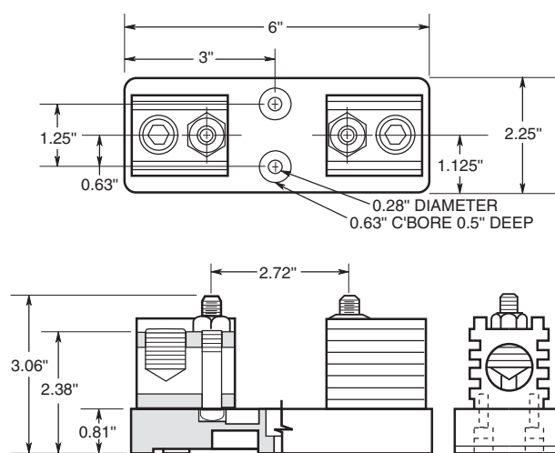
Figure 5. 201 to 400A
