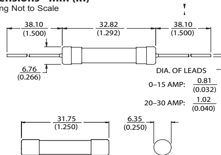
Dimensions - mm (in) Drawing Not to Scale
