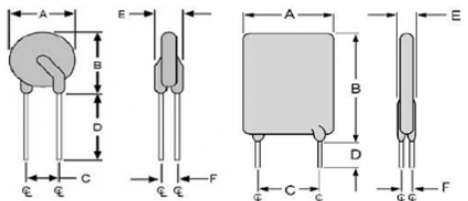
Fig.3 Lead Size : 20AWG Ø0.81 mm Diameter Fig.4 Lead Size : 20AWG Ø0.81 mm Diameter
