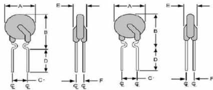
Fig.1 Lead Size : 24AWG Ø0.51 mm Diameter Fig.2 Lead Size : 22AWG Ø0.65 mm Diameter
