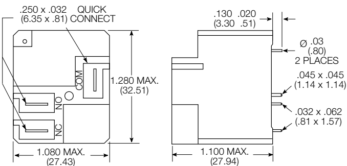
T9AS/V – Mounting and termination code 2
