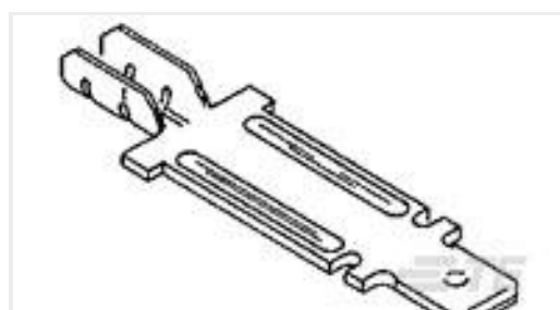
TE Part #41531 250 FASTON FLAG REC 18-12 AWG BR
