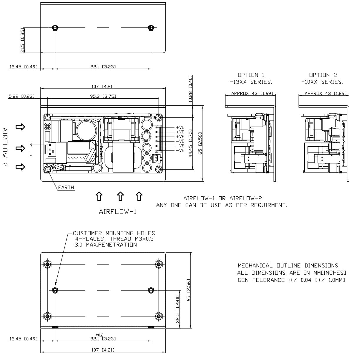
Figure 10. Mechanical Drawing – MEPG300-1XXX-L
