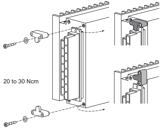
Fig. 44 Connector retention brackets HZZ01216-G (CRB-HKMS)
