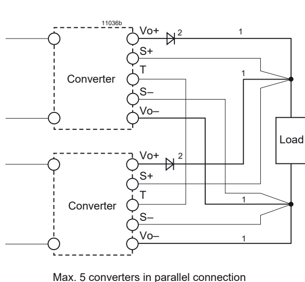
Fig. 34 Parallel connection of single-output models using option T with the sense lines connected at the load
