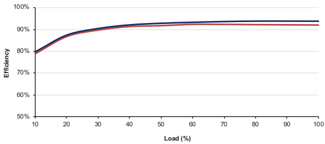
Figure 1 - ECH450PS12 (250W)
