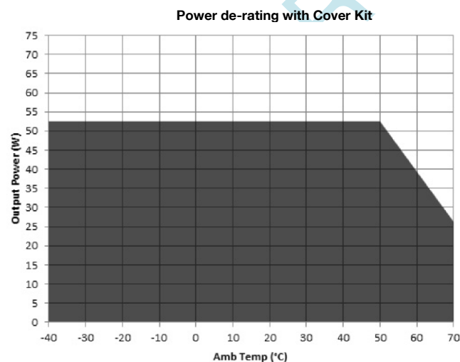
Figure 1. Derating Curves
