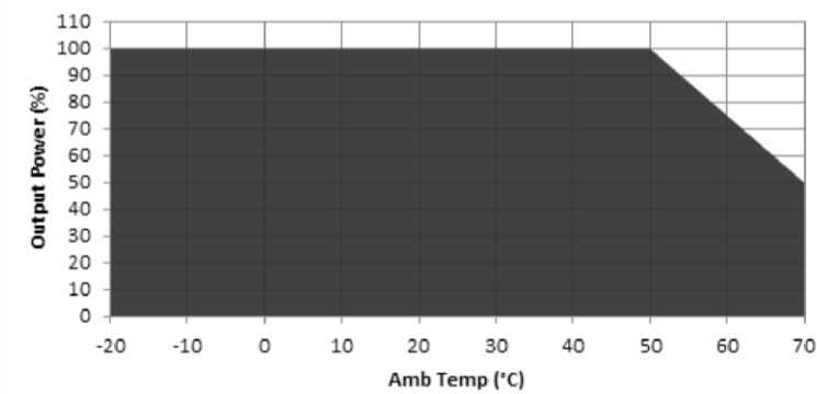
Figure 1. Derating Curve
