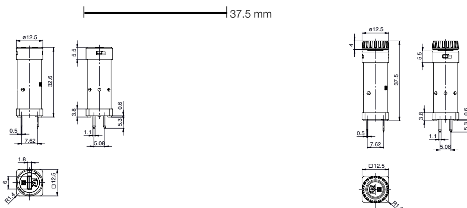
Variant Fingergrasp 3101.0045
