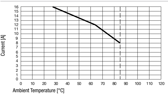
Variant 2 0751.0099, 0751.0100, 0751.0141 and 0751.0142
